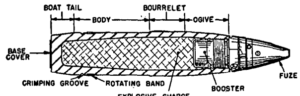
TYPICAL H.E. SHELL
